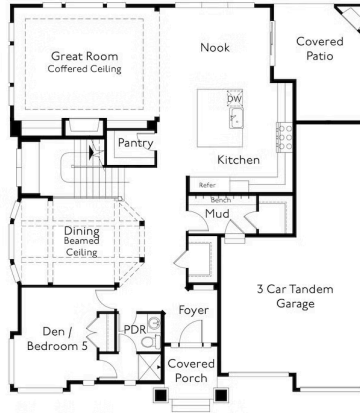
Main Level
